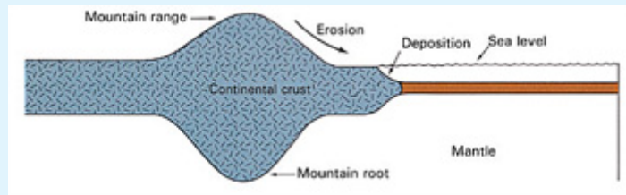
Figure 3: Another illustration shows how the mountains are peg-like in shape, due to their deep roots. (Earth Science, Tarbuck and Lutgens, p. 158.)
